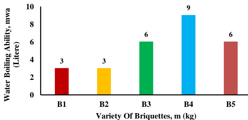
Figure 3. Variety of Briquettes to Water Boiling Ability
