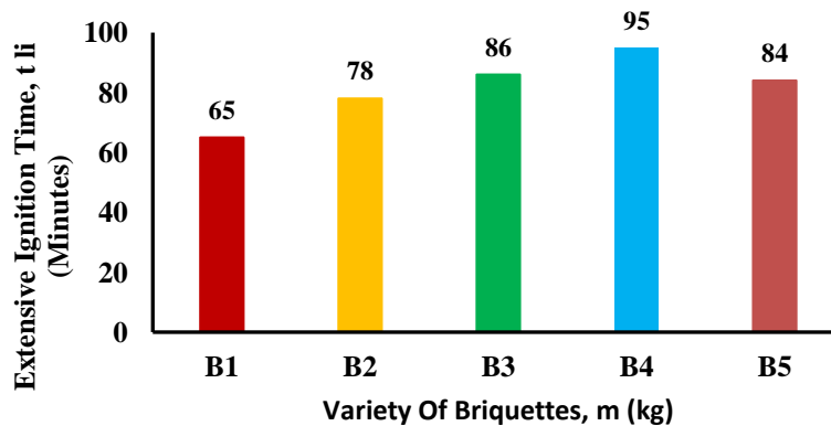
Figure 1. Extensive Ignition Time
