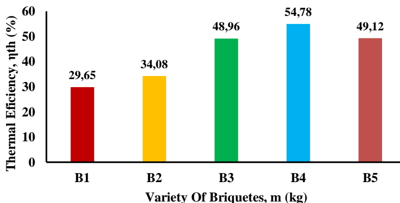
Figure 4. Shows Variety of Briquettes to thermal Efficiency
