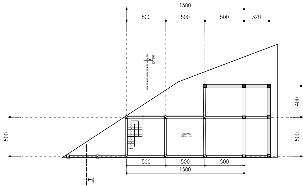
01 DENAH BASEMENT I FFL - 11.15 (EL 69.15) - SCALE 1 : 100
