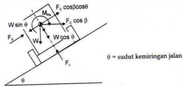
Gambar 2. Analisa CG (Center of Gravity)
