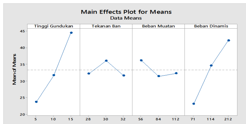
Gambar 6. Main Effects Plot of Means pada nilai Getaran Acceleration RMS Suspensi
