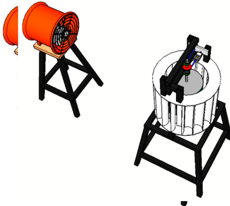
Gambar L. 4 Cylindrical guide vane diameter 400mm
