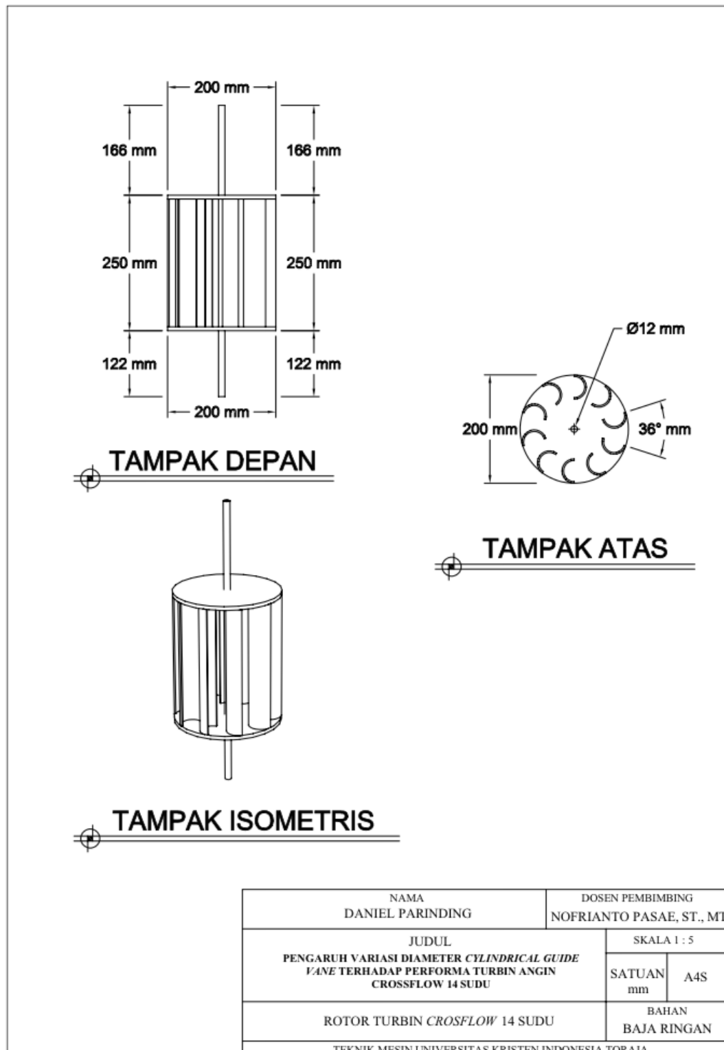
Gambar L. 15 Rotor Turbin Crossflow 14 Sudu
