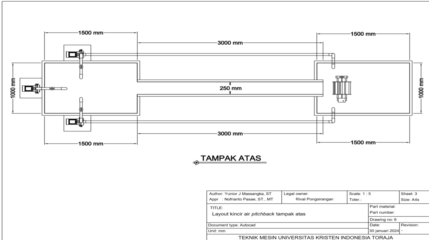
Gambar L.13 Layout kincir airpitchback tampak atas
