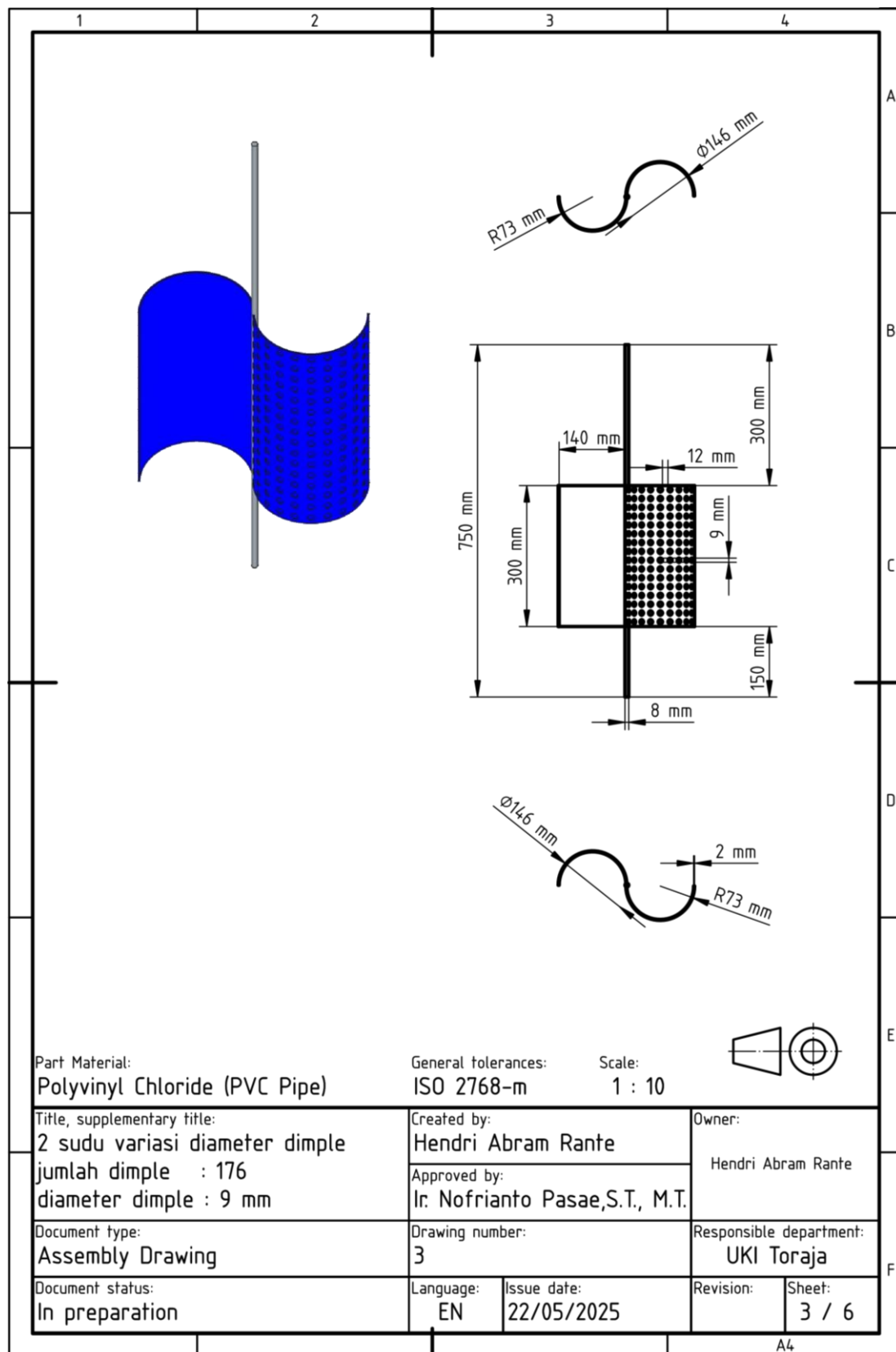
Gambar L.5 Dua sudu diameter dimple 9 mm
