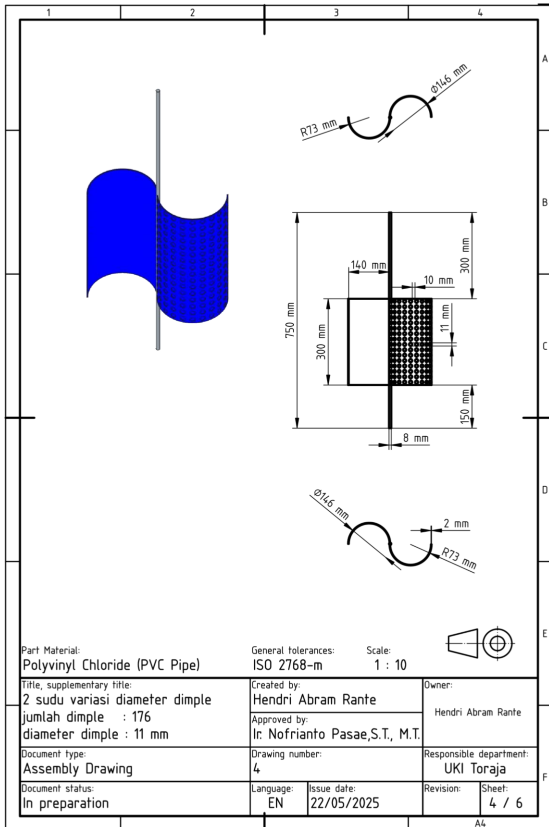
Gambar L.6 Dua sudu diameter dimple 11 mm
