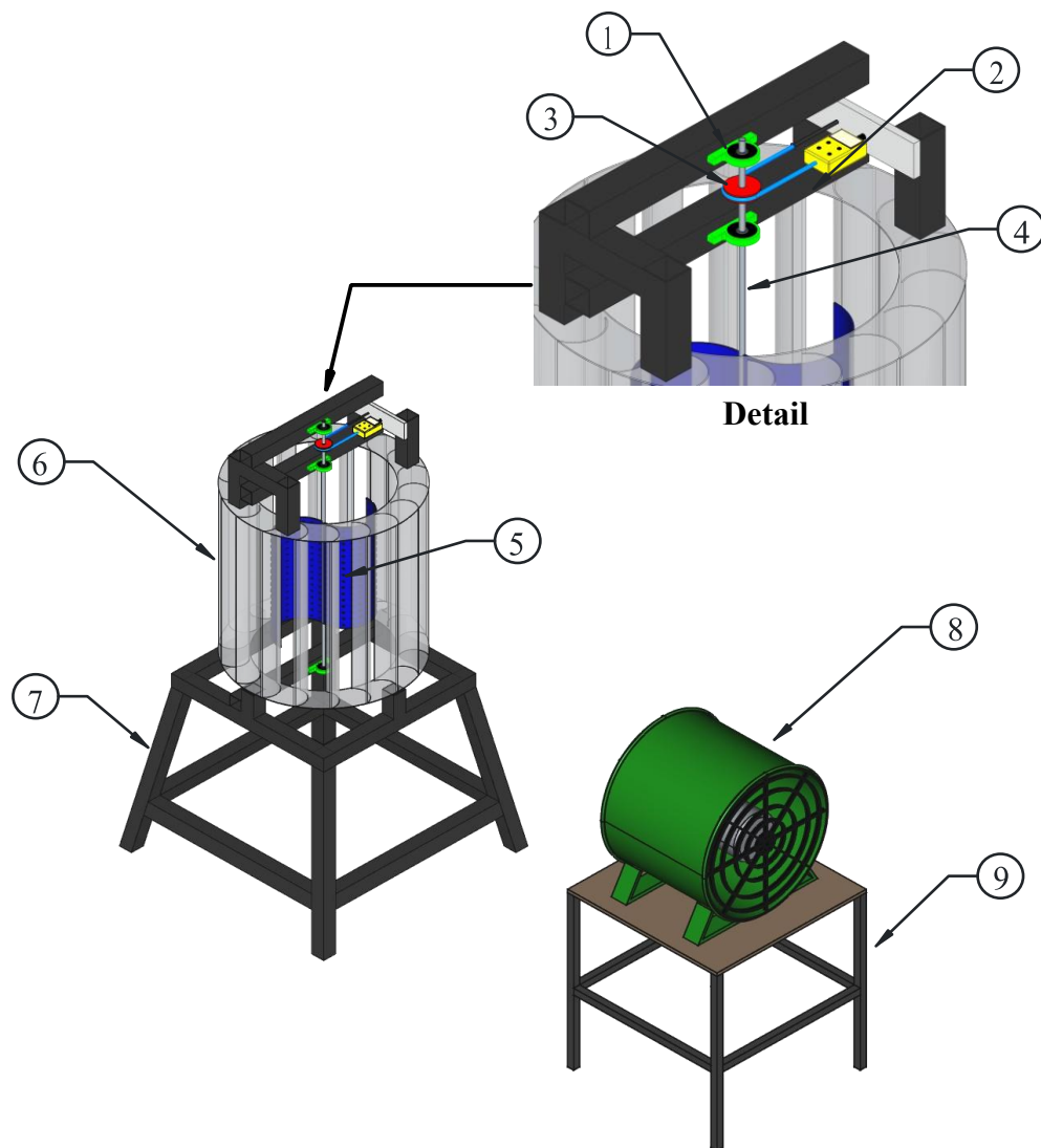
Gambar L.1 Layout turbin angin Savonius 2 sudu variasi diameter dimple
