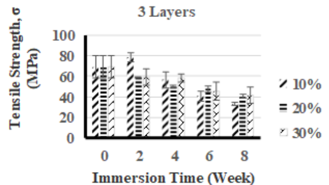
Fig 10. Graph of 2, 4, 6, 8 weeks of immersion time variation on the tensile strength of 3-layer bamboo woven reinforced composite material and 10, 20, 30% salinity percentage variation
