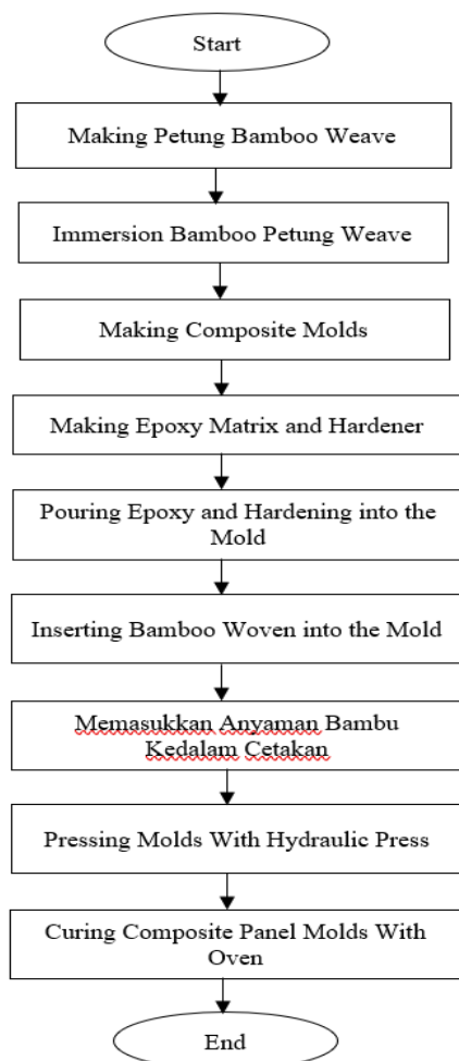
Fig. 6. Manufacturing process flow diagram composite panel
